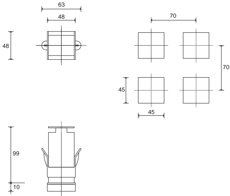
Dimensions: 48x48mm (1/16DIN )
