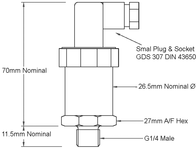
Small Plug & Socket IP65, GDS 307 DIN 43650 \varnothing
